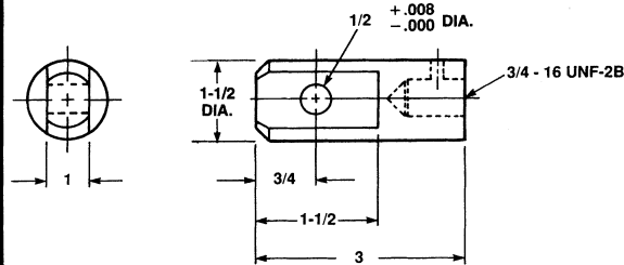
Clevis End (Optional) SK2800-4-2A
