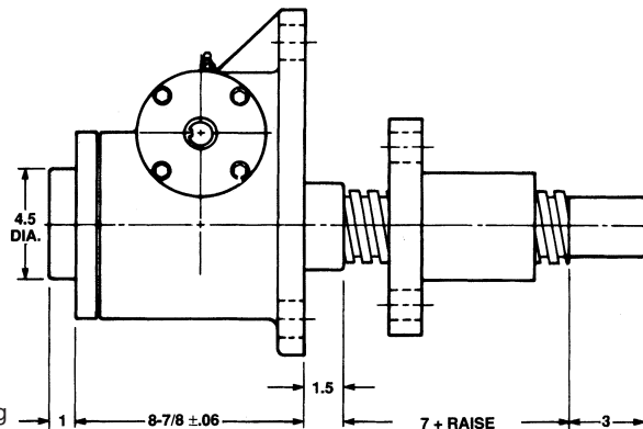
Upright Rotating: UM-9026
